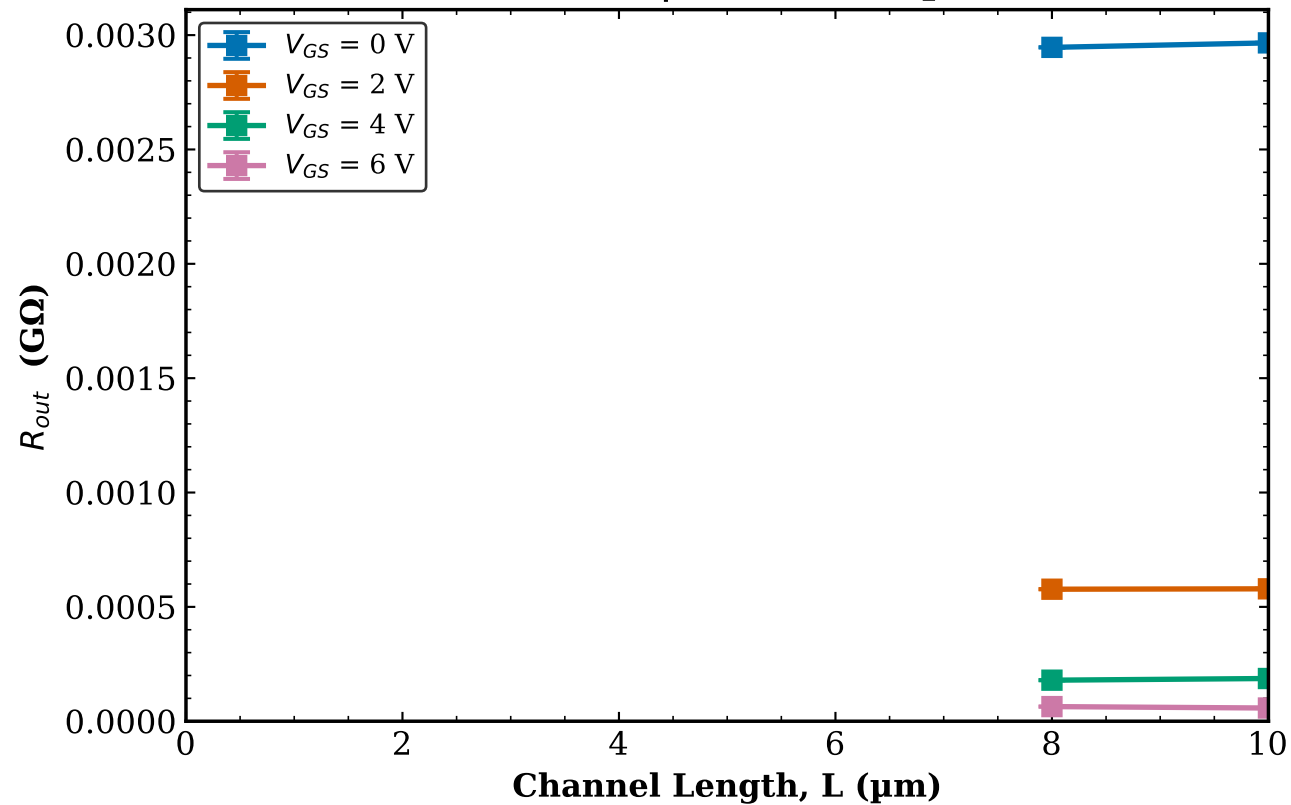
TFT1 Transistor 1 R_{out} vs L | W = 1000 \mu\text{m}
